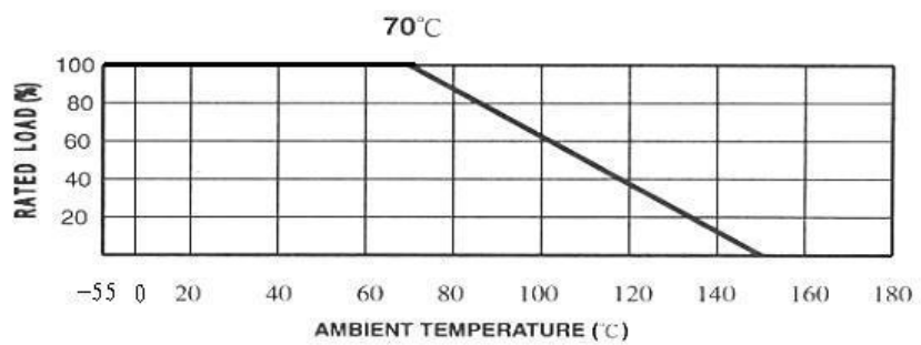
FIG.1 DERATING CURVE
